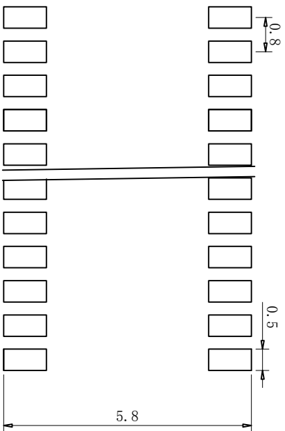
PCB LAYOUT
