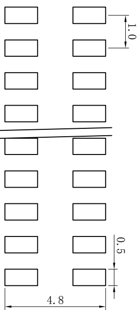
PCB LAYOUT
