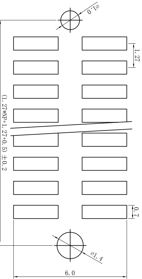
PCB LAYOUT
